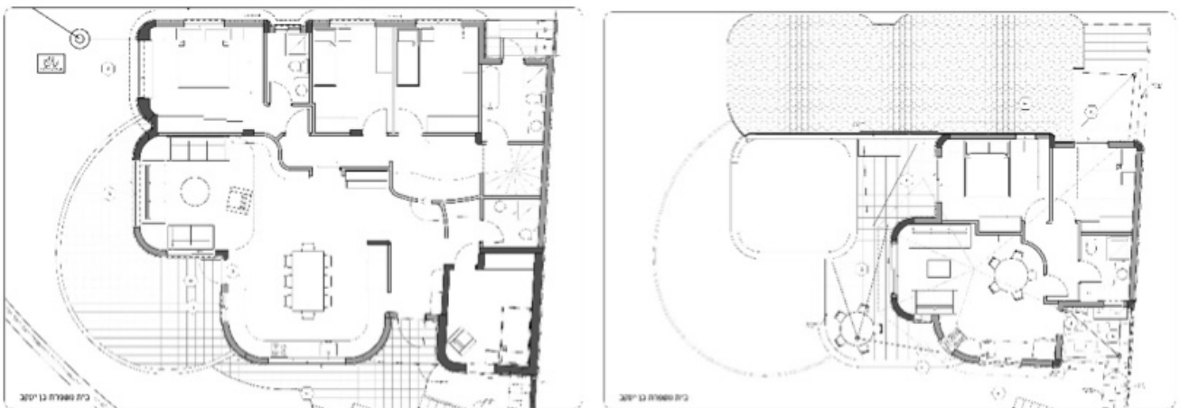
Plans of the two floors © Dror Zur
